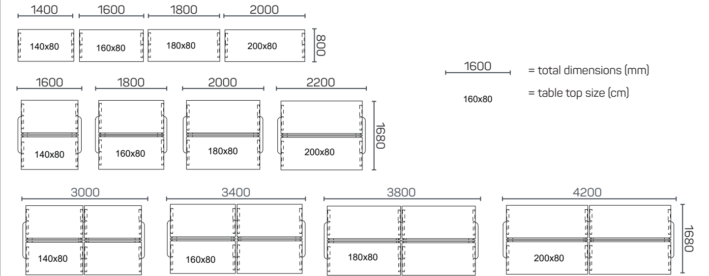
ParQ - sizes (+ total dimensions configuration)
